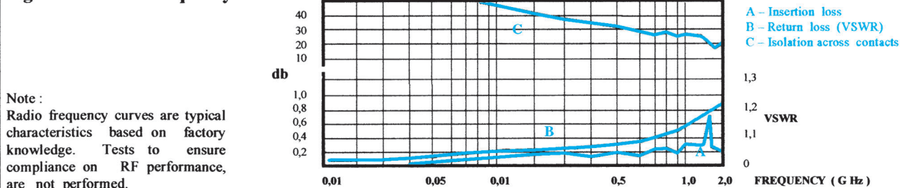
Figure 1 - Radio Frequency Curves
